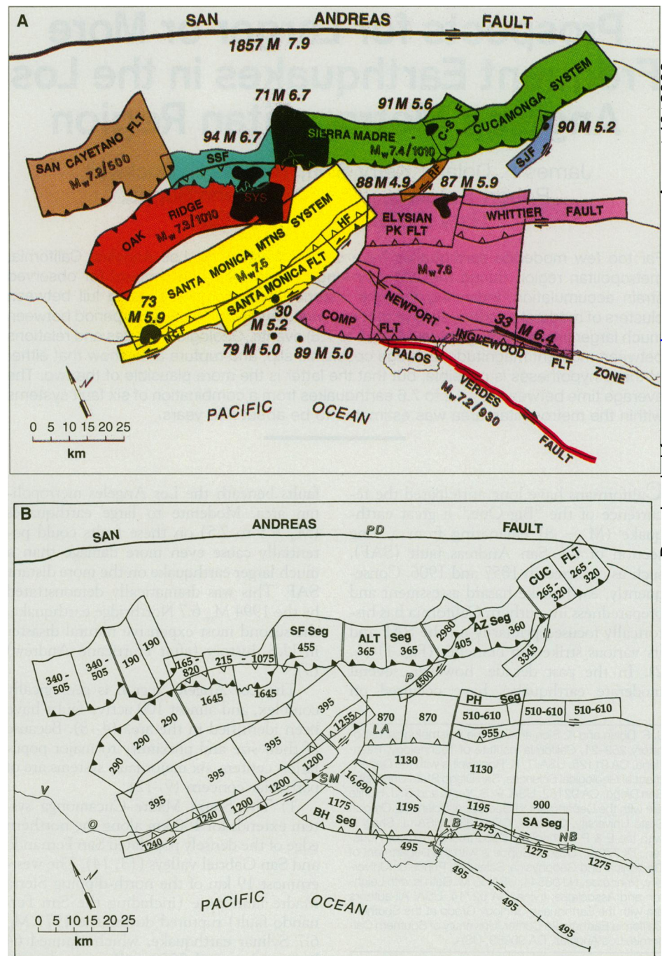
Fig. 1. (A) Historical earthquake ruptures and proposed large earthquake sources within the greater Los Angeles metropolitan area. Black areas denote surface projections of rupture planes of selected moderate historic earthquakes (6, 35–40, 65–67). Date and magnitude ( M_w ) of each earthquake are also shown. Historic ruptures on vertical strike-slip faults (1857 and 1933 earthquakes) are shown as heavy black lines. Polygons represent map projections of nonvertical fault planes. Thin lines denote near-vertical faults. Intermediate-width lines outline major fault systems that we consider could cause large earthquakes ( M_w 7.2 to 7.6). Solid bars denote thrust faults that break the surface; bars point down-dip. Open bars represent the upper edge of blind thrust fault ramps; bars point down-dip. Predominantly strike-slip faults are shown by double arrows along the surficial trace of each fault. Maximum credible earthquakes and their average recurrence intervals are shown for each fault system (for example, M_w 7.4/1010 on the Sierra Madre system indicates a recurrence interval of approximately 1010 years for a M_w 7.4 earthquake rupturing the entire system). Comp FLT, Compton fault; C-SF, Clamshell-Sawpit fault; HF, Hollywood fault; MCF, Malibu Coast fault; RF, Raymond fault; SJF, San José fault; SSF, Santa Susana fault. (B) Map showing the 51 potential, moderate ( M_w 6.5 to 6.8; average M_w 6.7) earthquake sources within the metropolitan region that we used in our moderate-earthquake scenario. The number within each earthquake source area denotes the approximate average recurrence interval (in years) for a moderate earthquake from each source region. In this scenario, for example, the source of the Northridge earthquake produces a M_w 6.7 event every 1645 years. Double lines denote geologically reasonable segment boundaries. ALT Seg, Altadena segment; AZ Seg, Azusa segment; BH Seg, Baldwin Hills segment; CUC FLT, Cucamonga fault; LA, downtown Los Angeles; LB, Long Beach; NB, Newport Beach; O, Oxnard; P, Pasadena; PD, Palmdale; PH Seg, Puente Hills segment; SA Seg, Santa Ana segment; SF Seg, San Fernando segment; SM, Santa Monica; V, Ventura.
